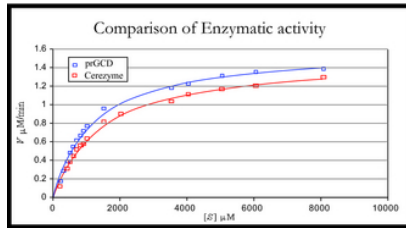
Figure 1: prGCD and Cerezyme Enzymatic Activity
