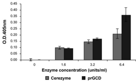
Figure 2: prGCD and Cerezyme Cellular Uptake
